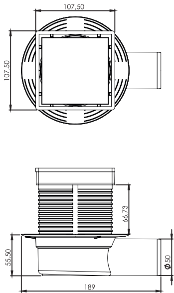
10*10 Yatay Sifon
