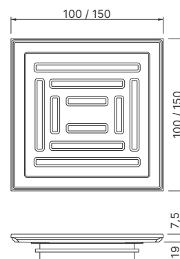
Odor Trap 30 mm water seal Y.8163.30
